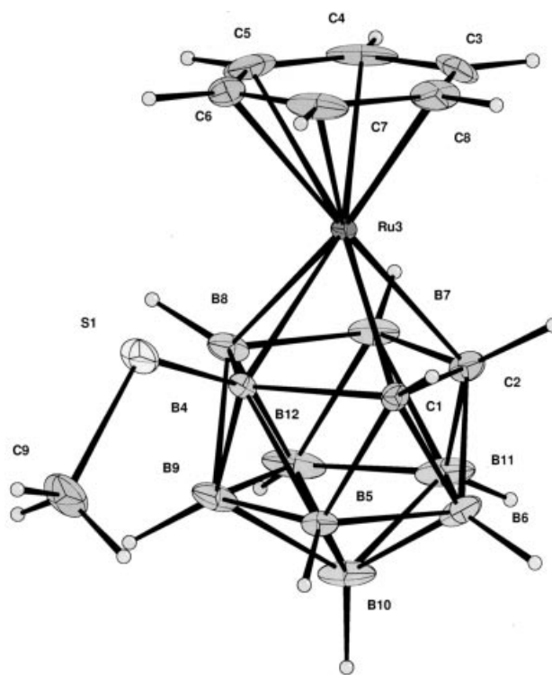
Figure 4. Molecular structure of 8 (thermal ellipsoids shown at the 50% probability level). Selected interatomic distances [Å]: Ru3–C1 2.153(2), Ru3–C2 2.163(2), Ru3–B4 2.202(3), Ru3–B7 2.198(3), Ru3–B8 2.215(3), Ru3–C3 2.228(3), Ru3–C4 2.199(3), Ru3–C5 2.188(3), Ru3–C6 2.199(3), Ru3–C7 2.214(3), Ru3–C8 2.235(3), C1–C2 1.627(3), C2–B7 1.721(4), B7–B8 1.801(4), B4–B8 1.815(4), B4–S1 1.855(3), C9–S1 1.810(3).
