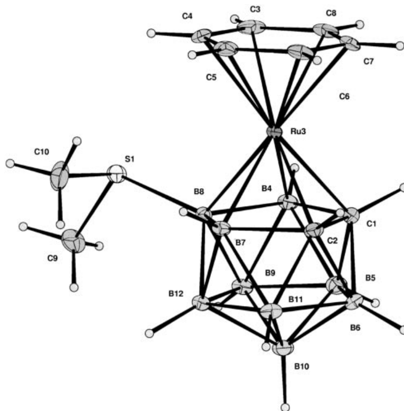
Figure 2. Molecular structure of [1a] PF 6 (thermal ellipsoids shown at the 50% probability level). The PF 6 − anion has been omitted for clarity. Selected interatomic distances [Å]: Ru3–C1 2.169(2), Ru3–C2 2.177(2), Ru3–B4 2.212(2), Ru3–B7 2.215(2), Ru3–B8 2.217(2), Ru3–C3 2.219(2), Ru3–C4 2.218(2), Ru3–C5 2.228(2), Ru3–C6 2.236(2), Ru3–C7 2.230(2), Ru3–C8 2.226(2), C1–C2 1.637(4), C2–B7 1.719(3), B7–B8 1.798(3), B4–B8 1.794(3), B8–S1 1.899(2).
