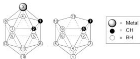
Scheme 1. Carborane numbering.
