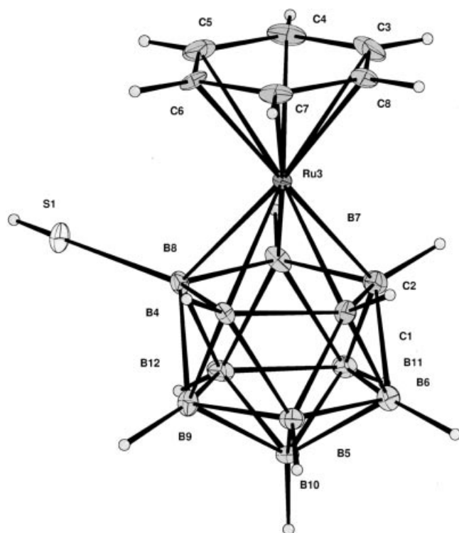
Figure 3. Molecular structure of 4 (thermal ellipsoids shown at the 50% probability level). Selected interatomic distances [Å]: Ru3–C1 2.157(3), Ru3–C2 2.164(3), Ru3–B4 2.202(3), Ru3–B7 2.198(3), Ru3–B8 2.215(3), Ru3–C3 2.242(3), Ru3–C4 2.229(4), Ru3–C5 2.206(3), Ru3–C6 2.197(3), Ru3–C7 2.221(4), Ru3–C8 2.238(3), C1–C2 1.644(4), C2–B7 1.727(4), B7–B8 1.810(4), B4–B8 1.808(4), B8–S1 1.836(3).
