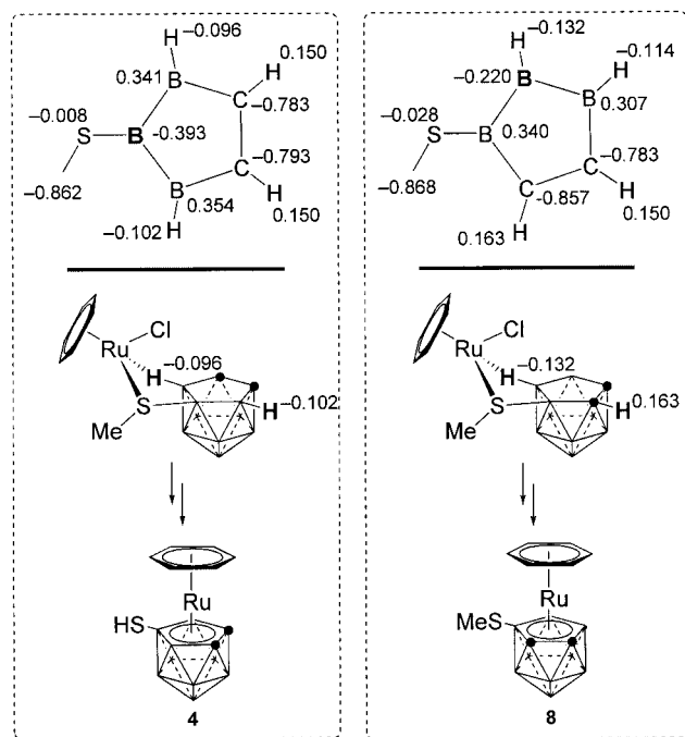
Scheme 5. Representation of the C_2B_3 faces of the nido -[10-MeS-7,8- C_2B_9H_{10} ] ^{2-} (left) and nido -[9-MeS-7,8- C_2B_9H_{10} ] ^{2-} ligands (right) and corresponding postulated exo-nido Ru species prior to the dealkylation reaction (below bold lines). Boron atoms in bold correspond to the B-8 vertex in the closo -ruthenacarborane complexes.
