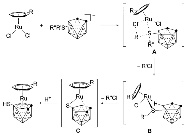
Scheme 3. Proposed pathway for the double dealkylation reaction.
