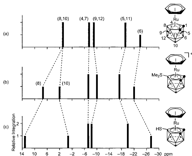
Figure 5. Representation of the ^{11}B\{^1H\} NMR spectra for complexes: (a) closo -[3-Ru( \eta^6 -benzene)-1,2- C_2B_9H_{11} ] (showing boron assignment); (b) [1a] PF _6 ; (c) 4 .
