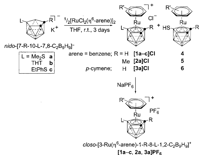
Scheme 2. Syntheses of new (arene)ruthenacarborane complexes.
