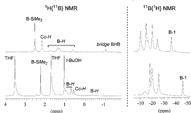
Figure 1. NMR monitoring for the deprotonation of nido -[10- \text{Me}_2\text{S} -7,8- \text{C}_2\text{B}_9\text{H}_{11} ]: (top) NMR spectra before addition of t BuOK (1.0 M solution in THF); (bottom) after addition of 1 equiv. of t BuOK (>99% nido -K[10- \text{Me}_2\text{S} -7,8- \text{C}_2\text{B}_9\text{H}_{10} ]).
