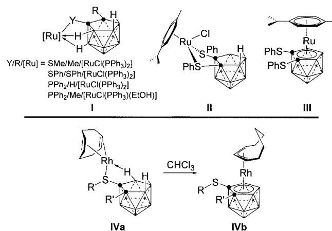
Scheme 4. Other selected ruthenium complexes and reactions.
